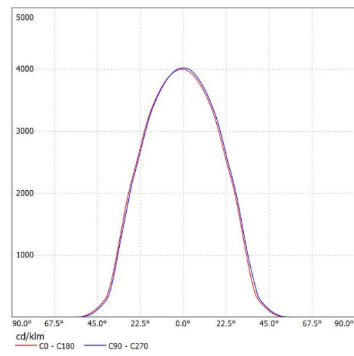
SL-07555B K:1.33cd/lm,LED:CXM-18
