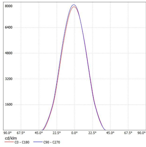
SL-07538B K:2.46cd/lm,LED:CXM-18
