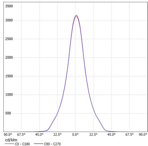
SL-07526B K:3.77cd/lm,LED:V15
