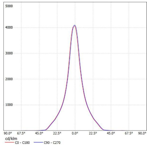
SL-07518B K:5.00cd/lm,LED:V15
