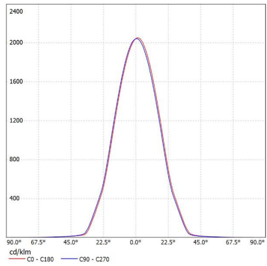
SL-07538B K:2.54cd/Im,LED:V15
