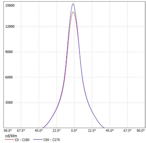
SL-07518B K:4.69cd/lm,LED:CXM-18
