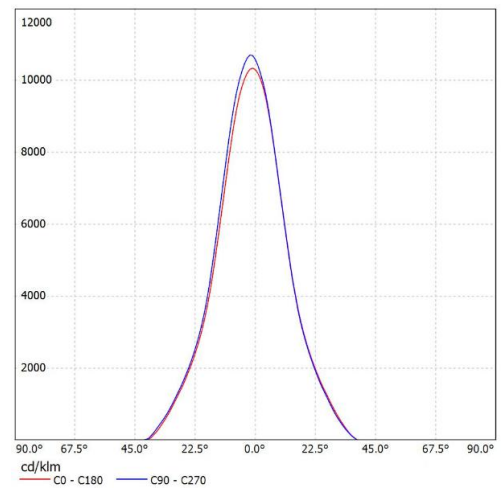
SL-07526B K:4.40cd/lm,LED:CXM-18
