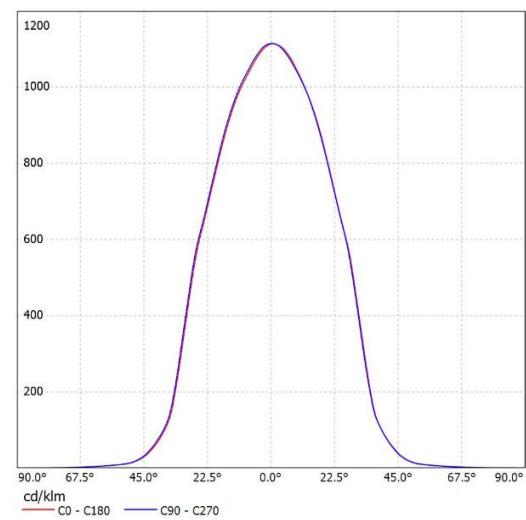
SL-07555B K:1.38cd/Im,LED:V15
